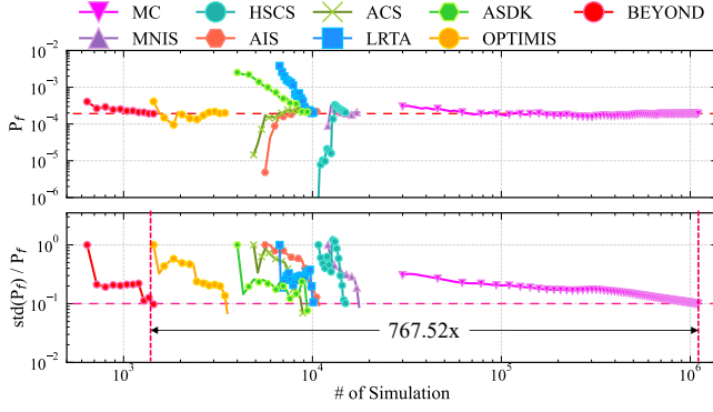
Figure 4: Failure rate estimation with FoM on OTA
