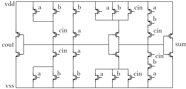
Figure 7: The structure of Adder circuit
