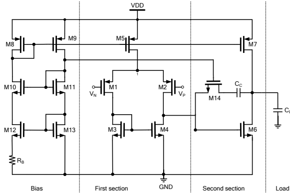
Figure 5: Operational Transconductance Amplifier Circuit
