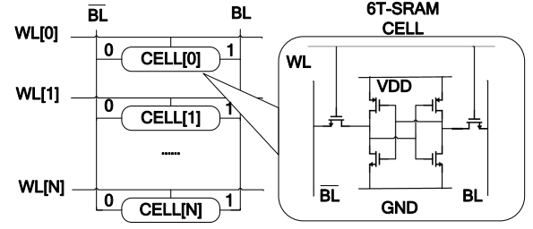
Figure 2: The structure of SRAM column circuit
