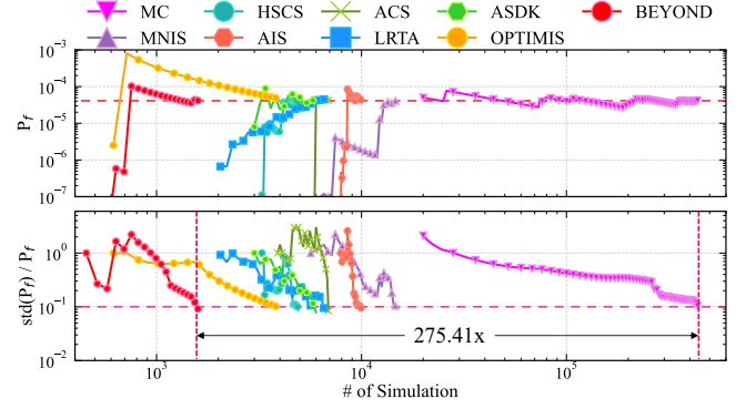
Figure 3: Failure rate estimation with FoM on 6T-SRAM
