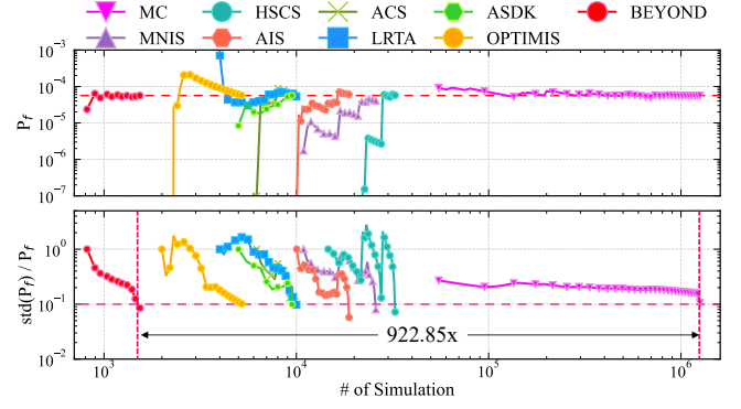
Figure 6: Failure rate estimation with FoM on 6-bit array
