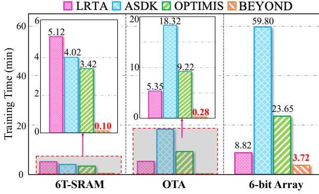
Figure 8: Model training time on three benchmark circuits
